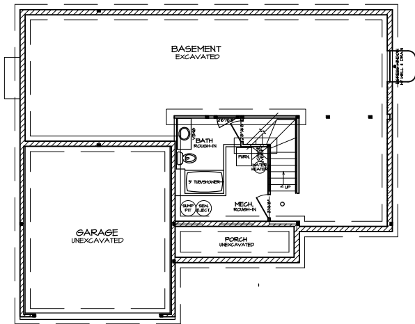
FOUNDATION PLAN
